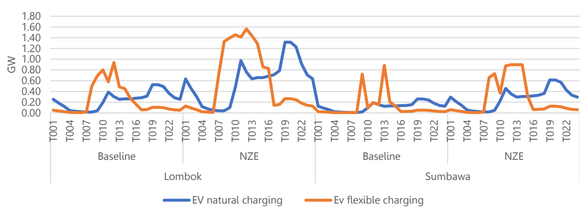
Figure 71: Comparison of the effect of flexible operation in EV charging.
