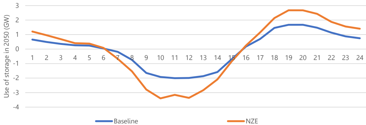
Figure 64: Average daily storage charging and discharging pattern for Nusa Tenggara Barat in 2050.
