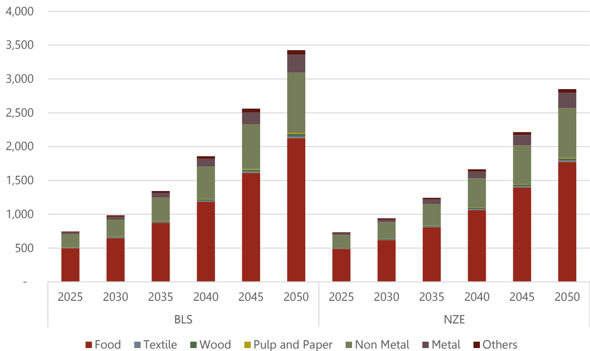
Figure 39. Industrial fuel consumption by process in NTB
