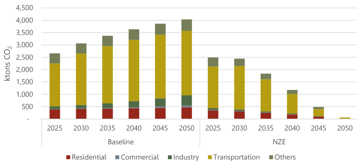
Figure 4: Total end-use CO 2 emissions by sector in NTB (excluding power sector)
