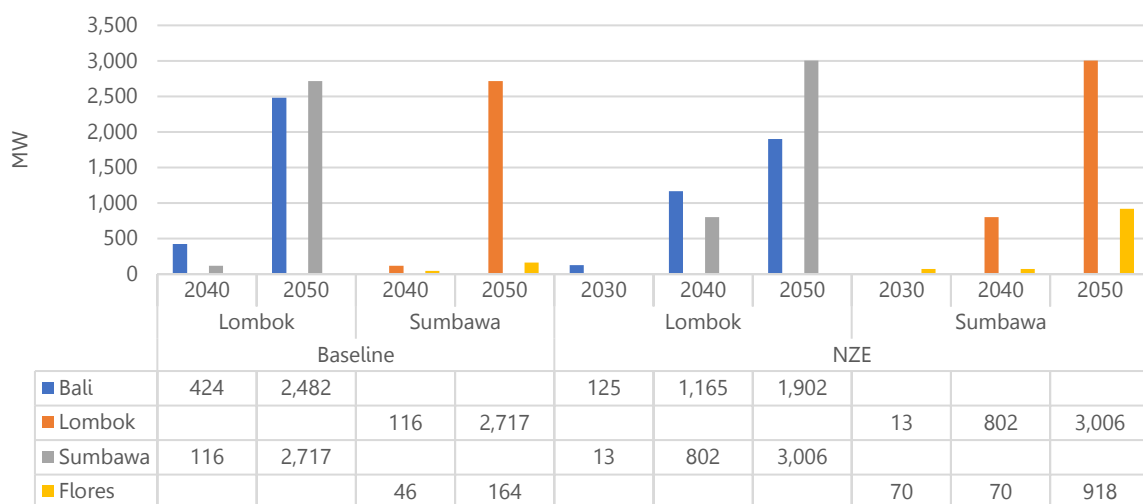
Figure 59: Installed power transmission capacity in the two scenarios.
