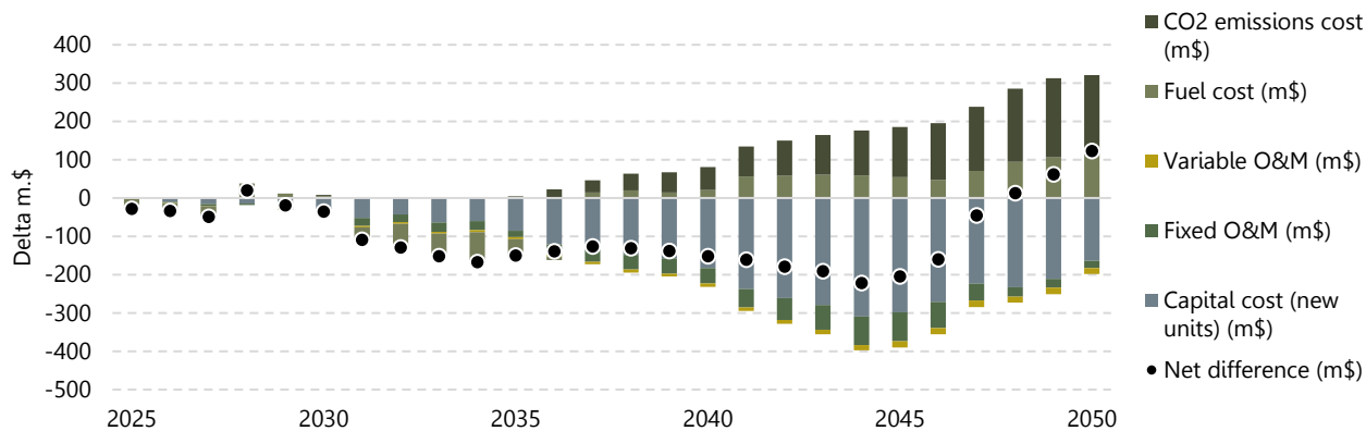
Figure 11: Overview of difference in system costs between NZE and Baseline including CO 2 costs for fossil fuels. Positive values mean lower system costs in NZE.
