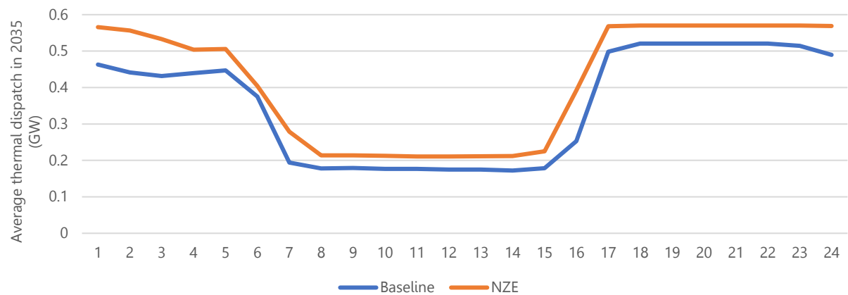
Figure 62: Average thermal dispatch in Nusa Tenggara Barat for 2035.
