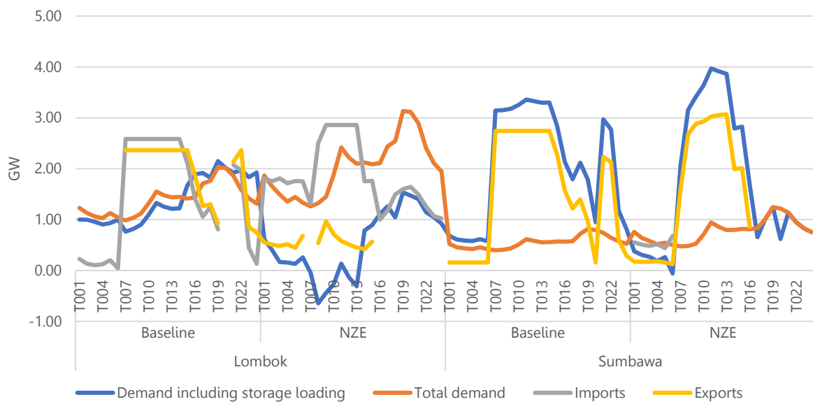
Figure 68: Comparison of demand, imports, and export with and without the effect of storages.
