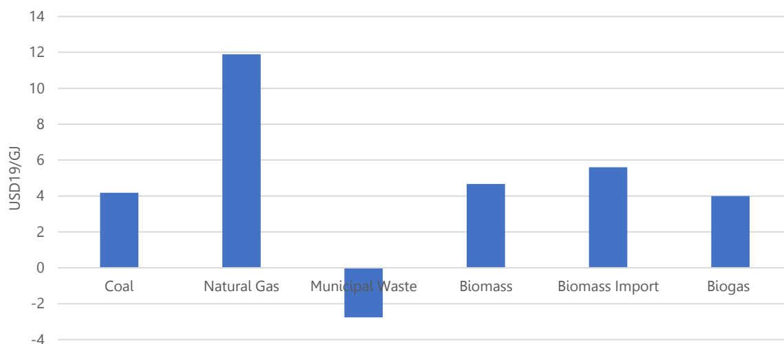
Figure 27 Fuel price assumed for all cases, for the period simulated development towards 2050 in in USD19.
