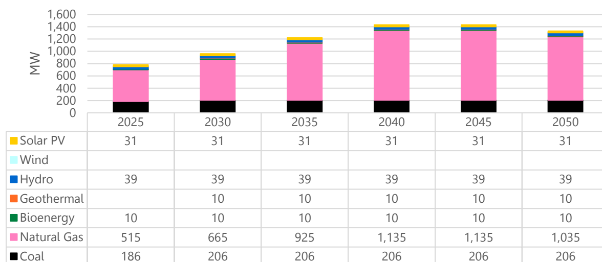
Figure 28: Existing and planned capacity expansion in Nusa Tenggara
