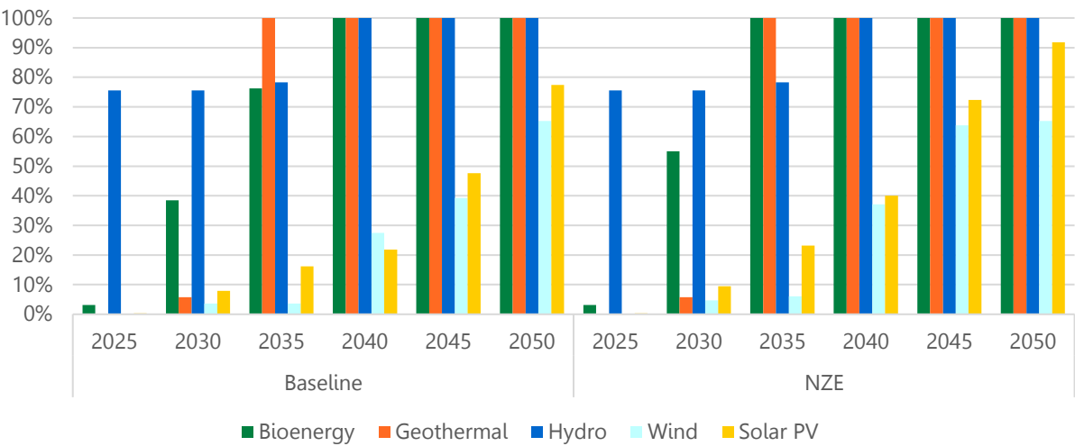
Figure 50: Share of installed capacity with respect to potential in the two scenarios.
