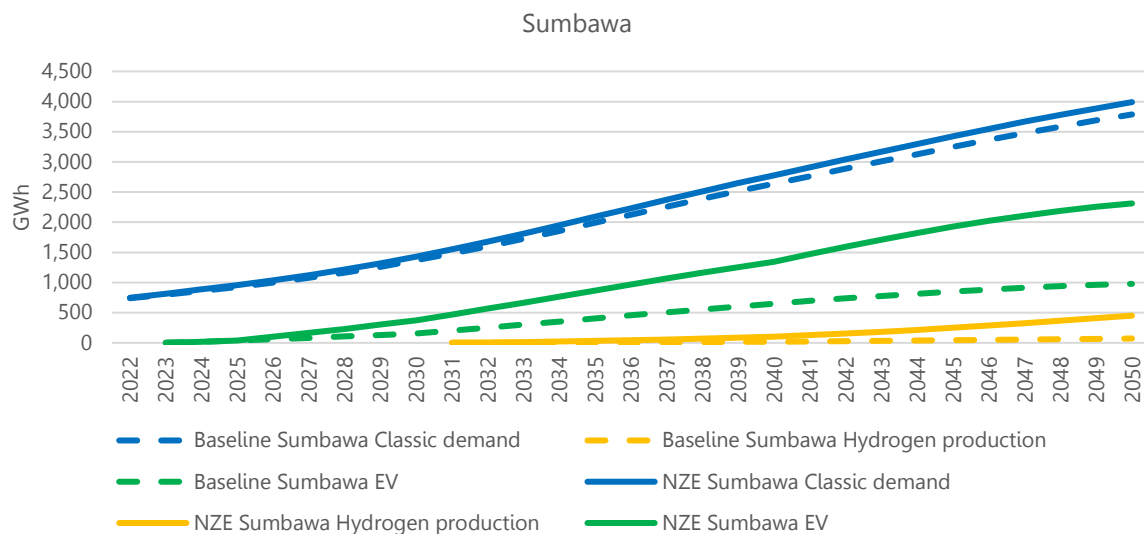
Figure 26 Electricity demand for Sumbawa in the baseline and NZE scenario.
