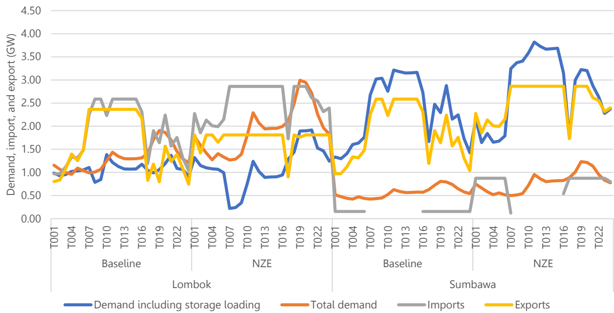
Figure 66: Comparison of demand, imports, and export with and without the effect of storages.
