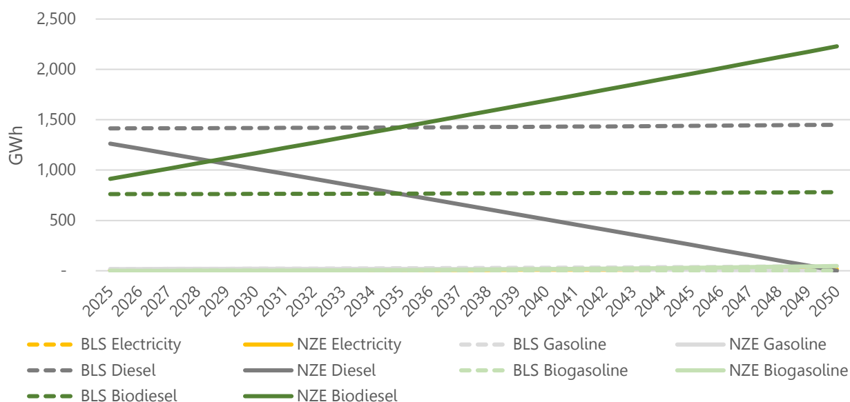
Figure 46: Others fuel consumption in Sumbawa.
