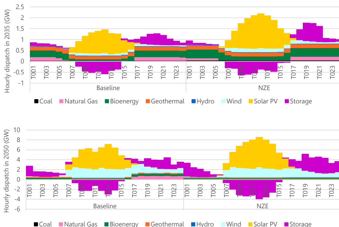
Figure 61: Hourly dispatch in Nusa Tenggara Barat for a day in an average week for the years 2023, 2035 and 2050.
