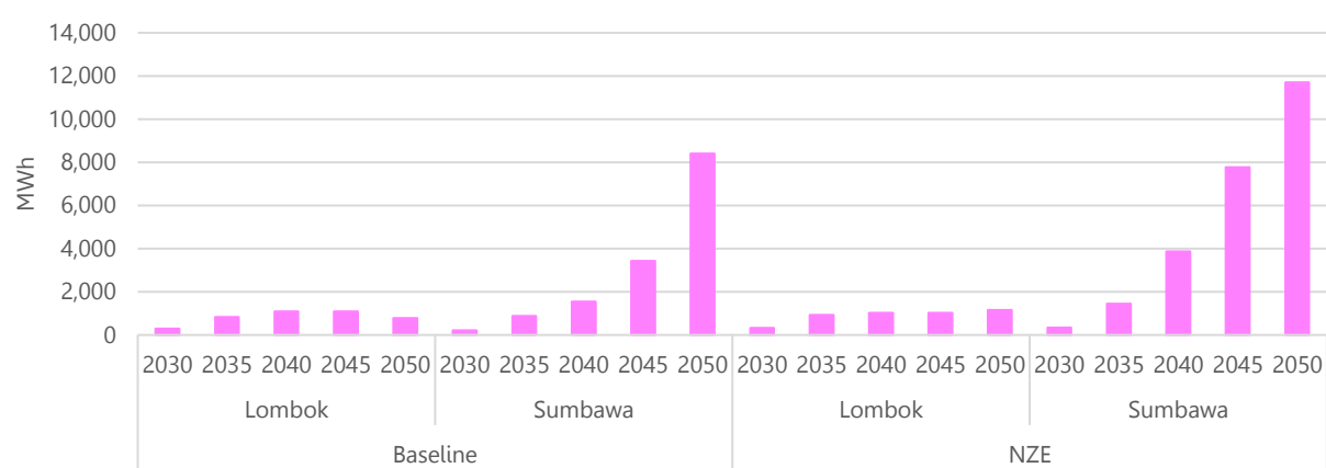
Figure 58: Overview of storage capacity in the two scenarios for Lombok and Sumbawa.
