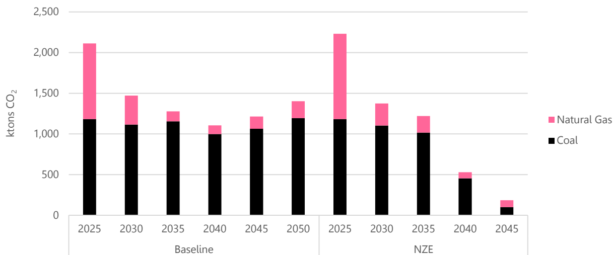
Figure 55: CO 2 emissions by fuel in the two scenarios.
