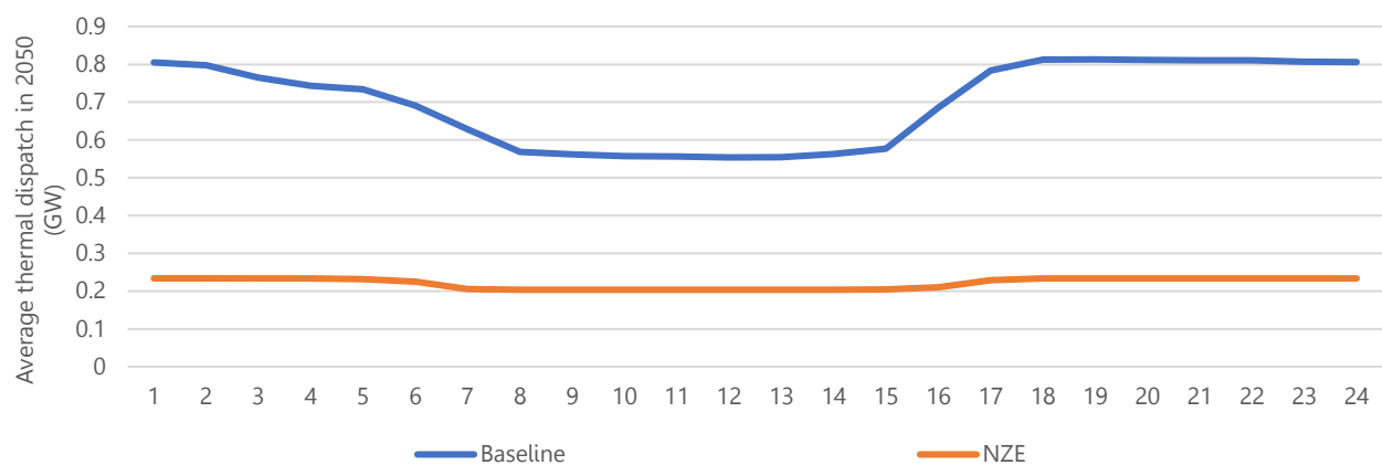
Figure 63: Average thermal dispatch in Nusa Tenggara Barat for 2050.
