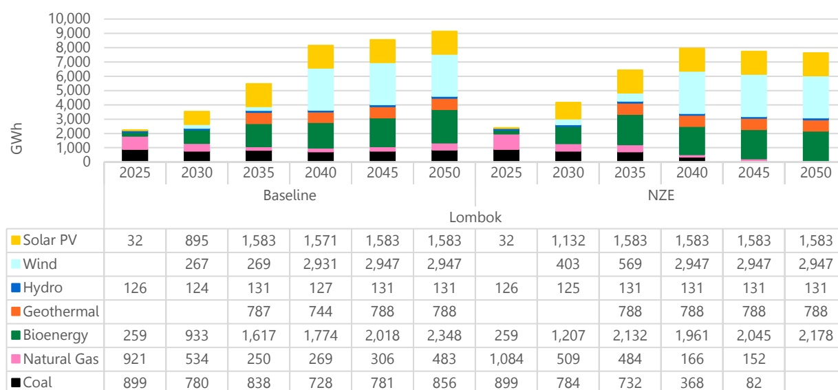
Figure 51: Overview of generation in the two scenarios for Lombok.
