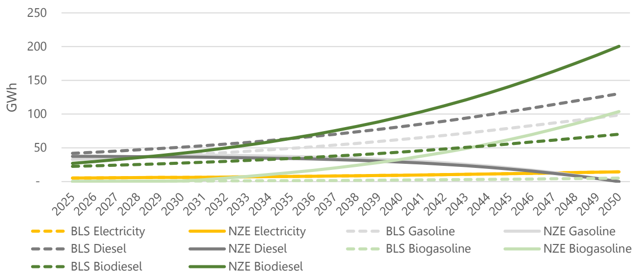
Figure 45. Others fuel consumption in Lombok
