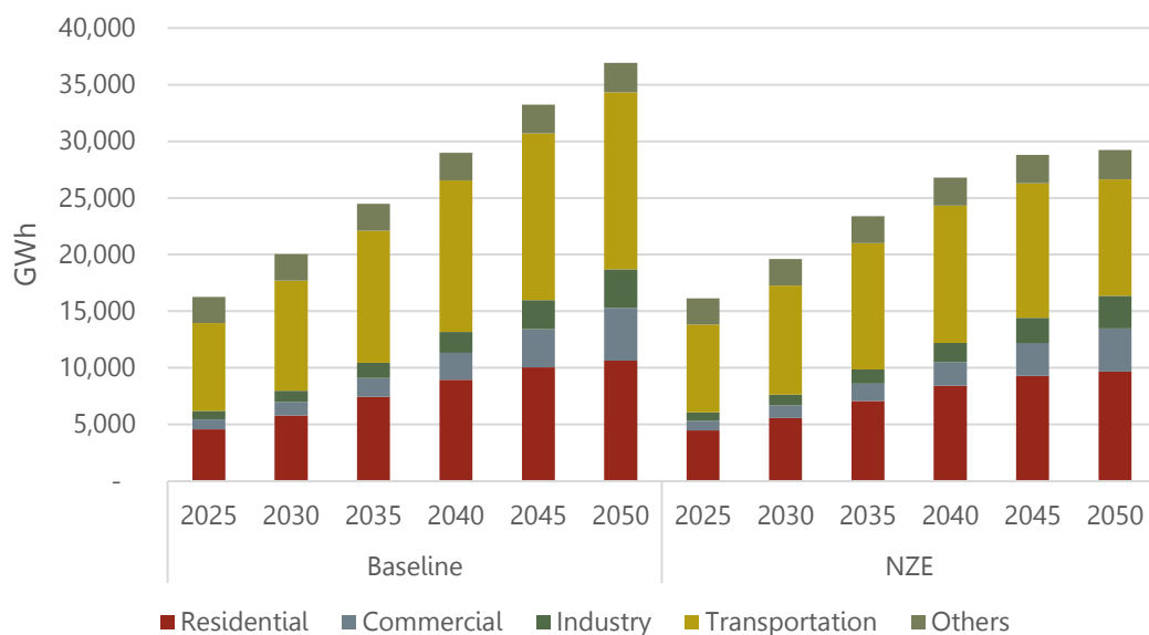
Figure 2: Total end-use energy demand by sector in NTB
