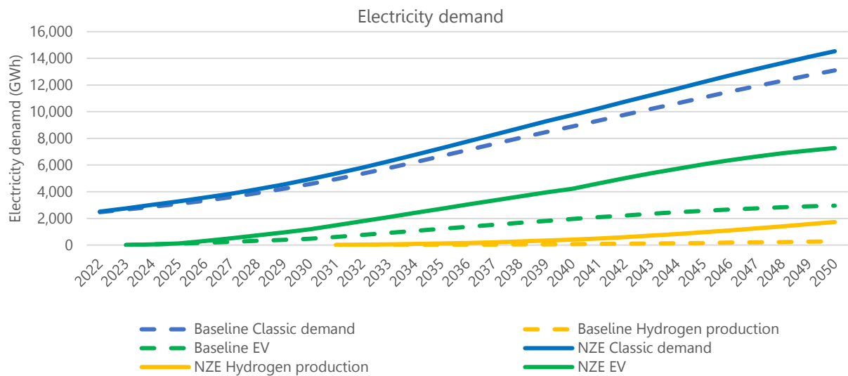
Figure 24 Electricity demand for Nusa Tenggara Barat as a whole in the baseline and NZE scenario.
