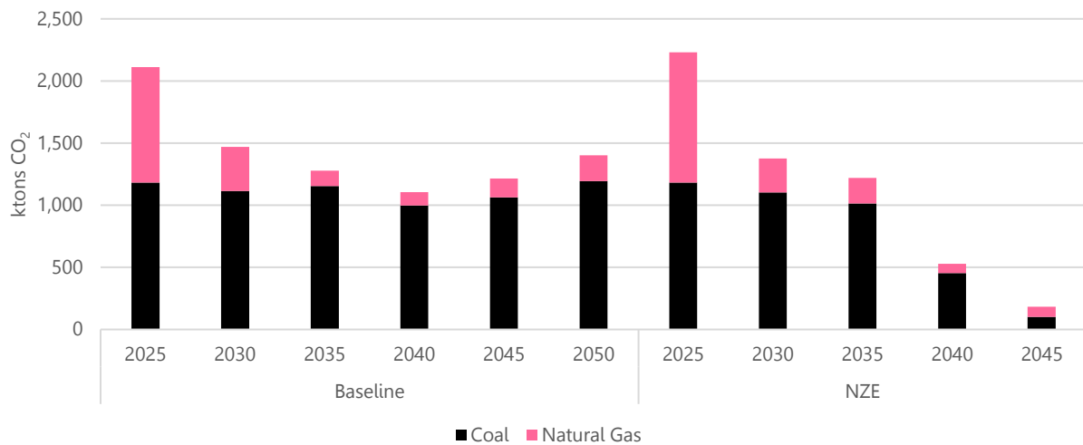
Figure 7: CO 2 emissions by fuel in the two scenarios.
