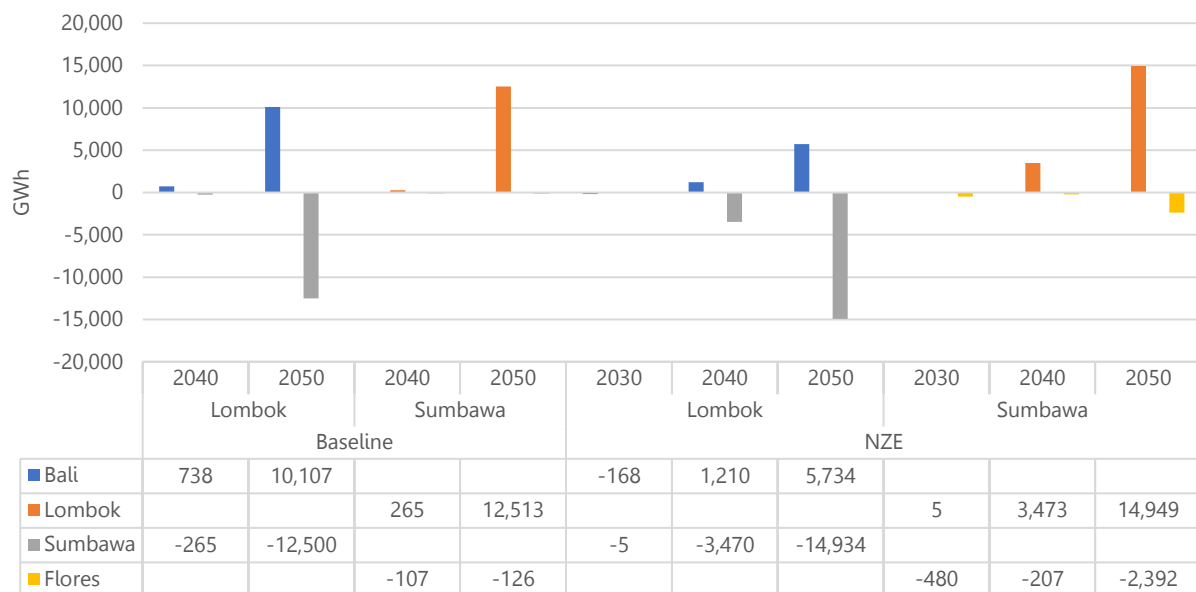
Figure 60: Overview of transmission flows to and from Lombok and Sumbawa.
