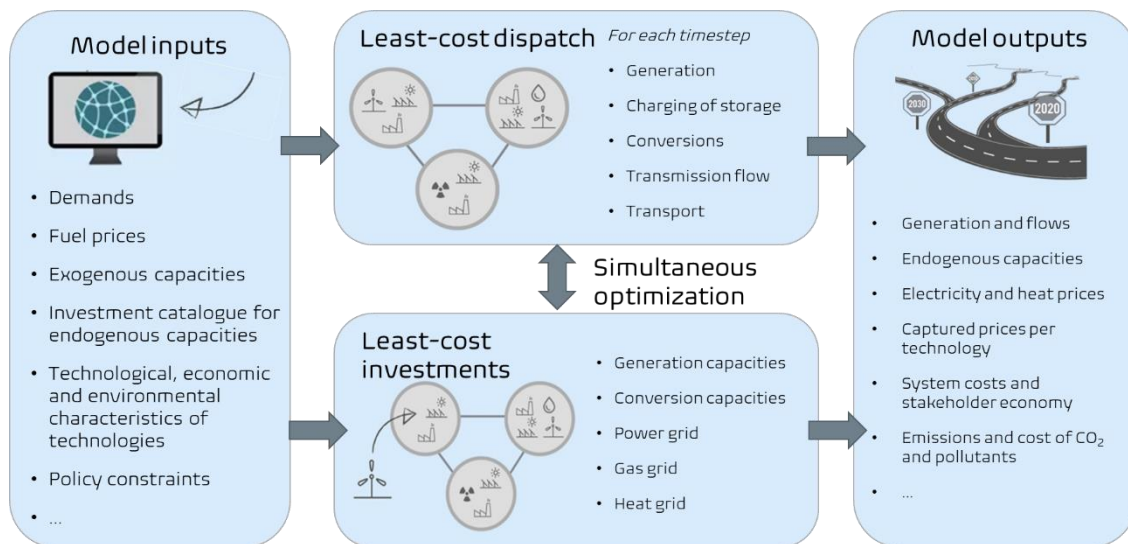
Figure 21: Overview of the Balmorel model's functionality, as well as key inputs and outputs.
