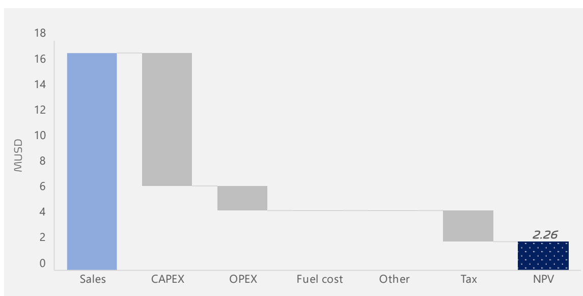
Figure 80: Overview of NPV for 50 MW Solar power capacity installed in Sumbawa-Bima in 2030 in NZE scenario.
