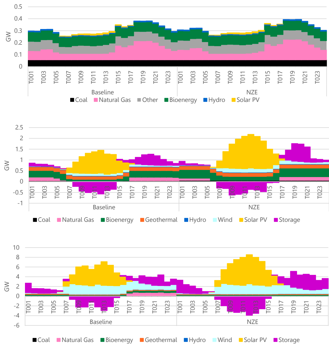
Figure 9: Dispatch in Nusa Tenggara Barat for the years 2023, 2035 and 2050.
