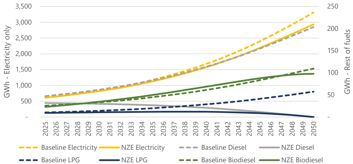
Figure 37. Commercial electricity consumption (left axis) and other fuel consumption (right axis) in Lombok
