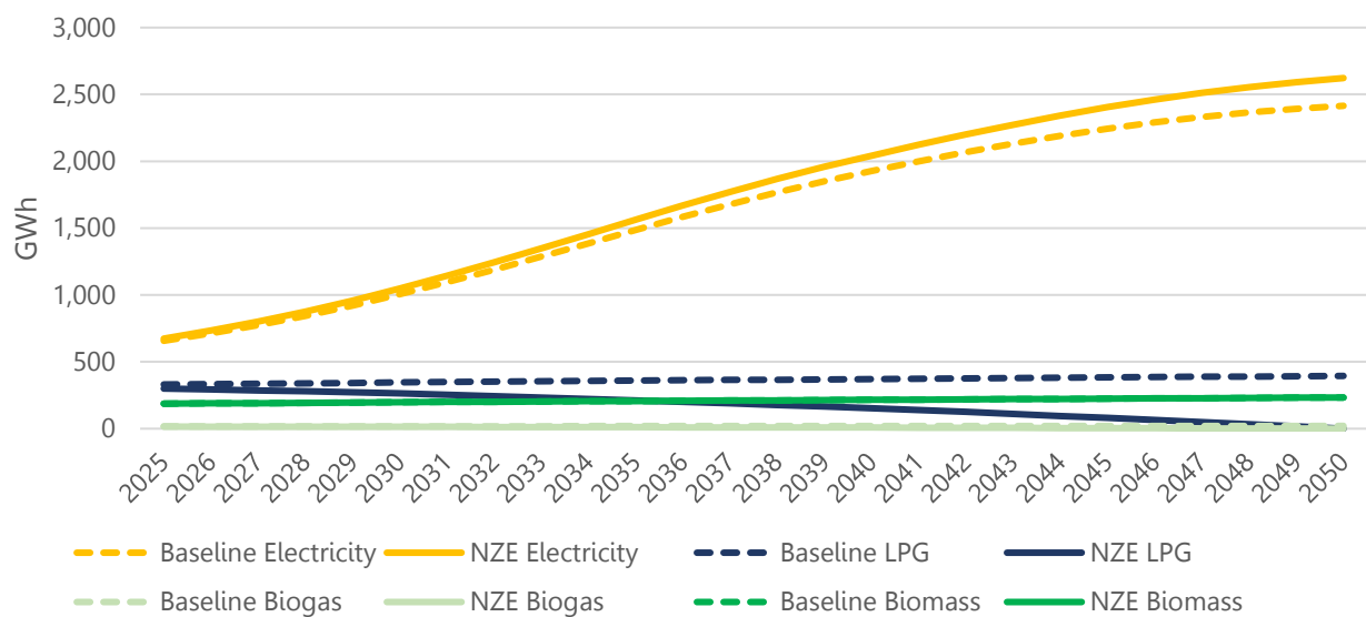
Figure 35. Residential fuel consumption in Sumbawa
