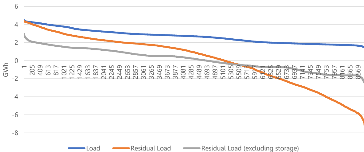
Figure 69: Duration curves in 2050 for the NZE scenario in the NTB province.
