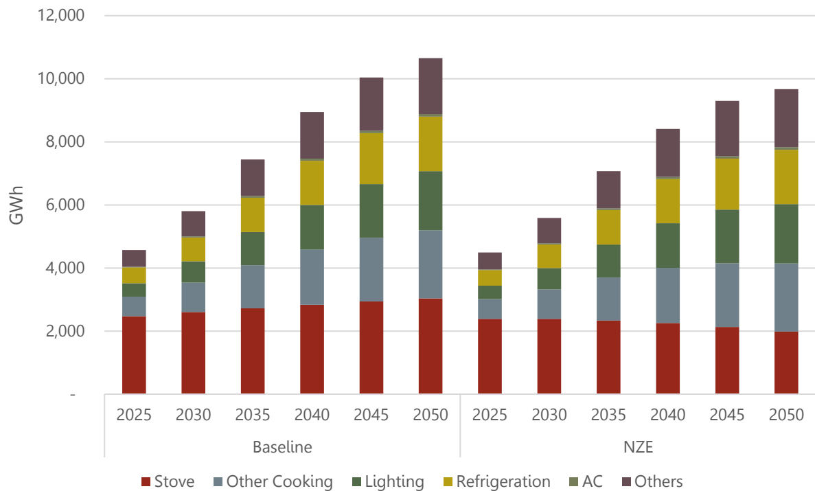
Figure 33. Residential total fuel consumption by application in NTB
