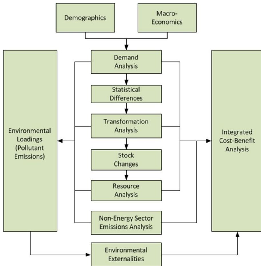
Figure 20: General LEAP calculations' structure (Source: SEI, USA)
