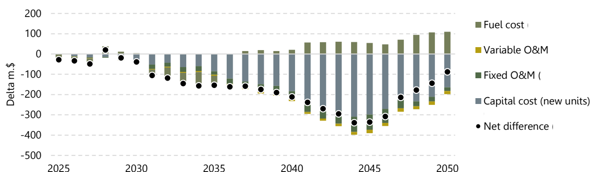
Figure 75: Overview of difference in system costs between the NZE and Baseline scenarios. Negative values mean higher system costs in NZE.
