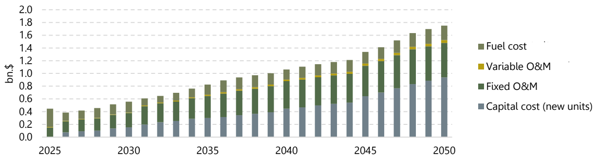
Figure 73: Annualized system costs for the Baseline scenario.
