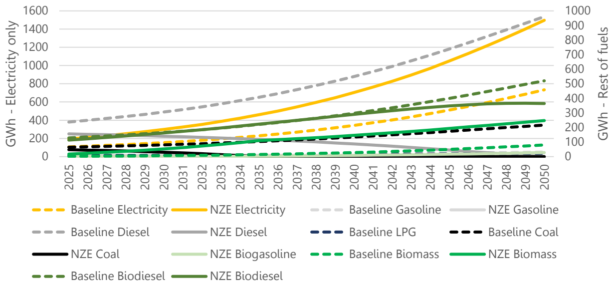
Figure 40. Industrial electricity consumption (left axis) and other fuel consumption (right axis) in Lombok
