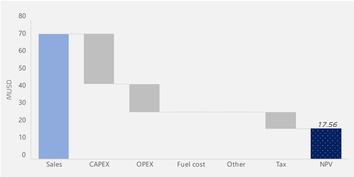
Figure 81: Overview of NPV for 50 MW onshore wind power installed in Lombok in 2026 in NZE scenario.
