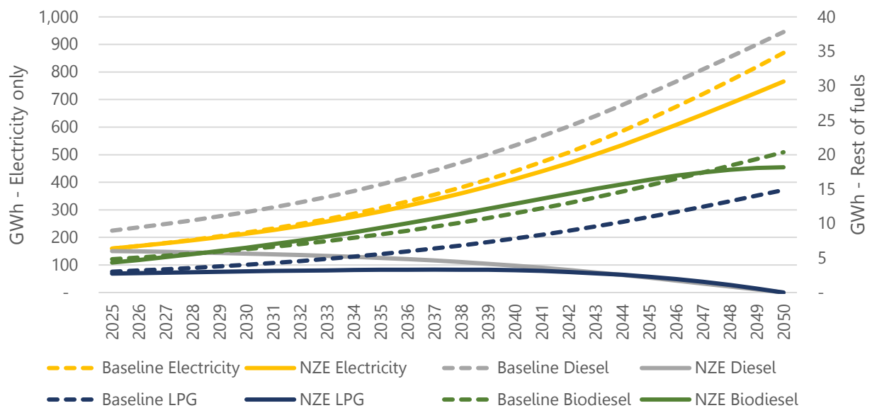
Figure 38. Commercial electricity consumption (left axis) and other fuel consumption (right axis) in Sumbawa
