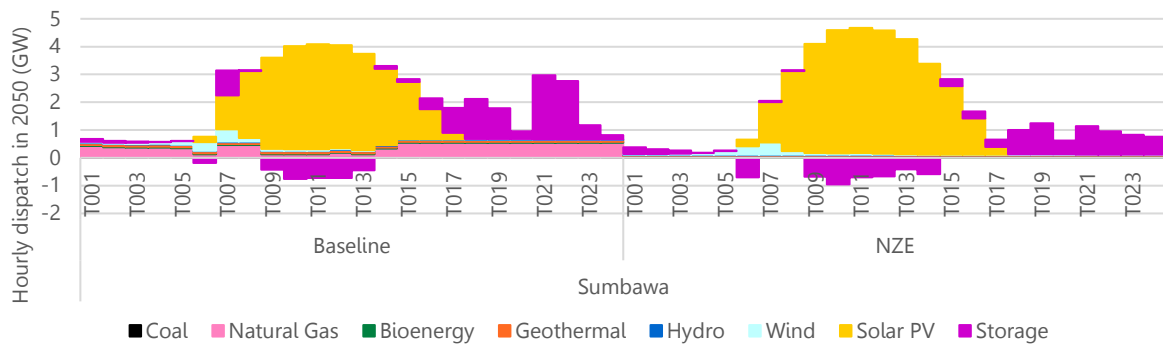
Figure 67: Daily dispatch in 2050 on a low VRE potential day.
