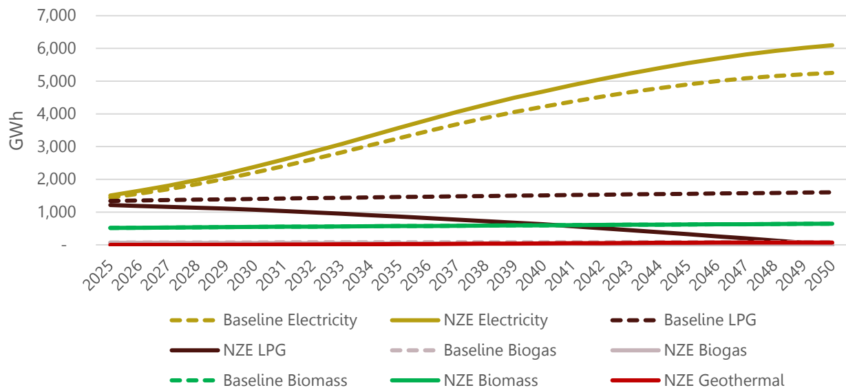
Figure 34. Residential fuel consumption in Lombok
