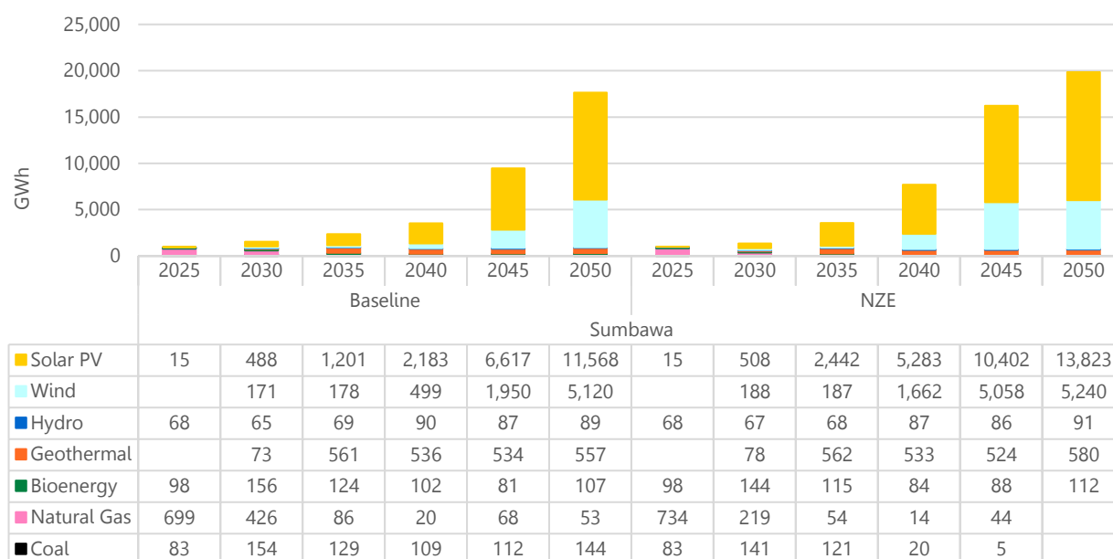
Figure 52: Overview of generation in the two scenarios for Sumbawa.
