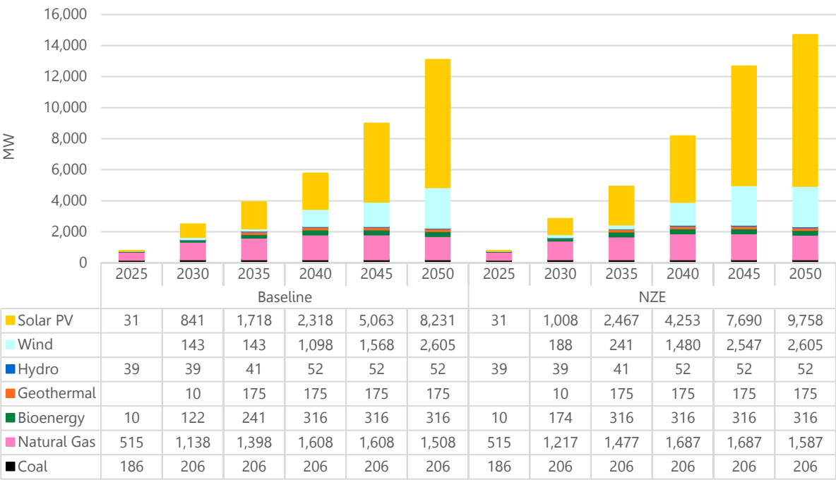
Figure 49 Installed capacity in Nusa Tenggara in the two main scenarios.
