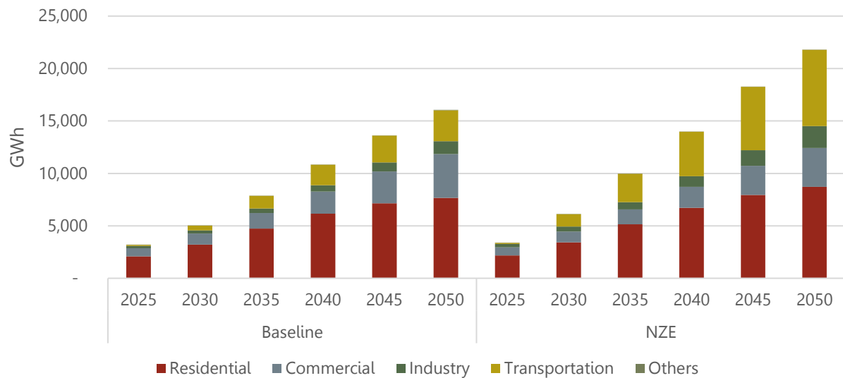
Figure 3: Total end-use electricity consumption by sector in NTB
