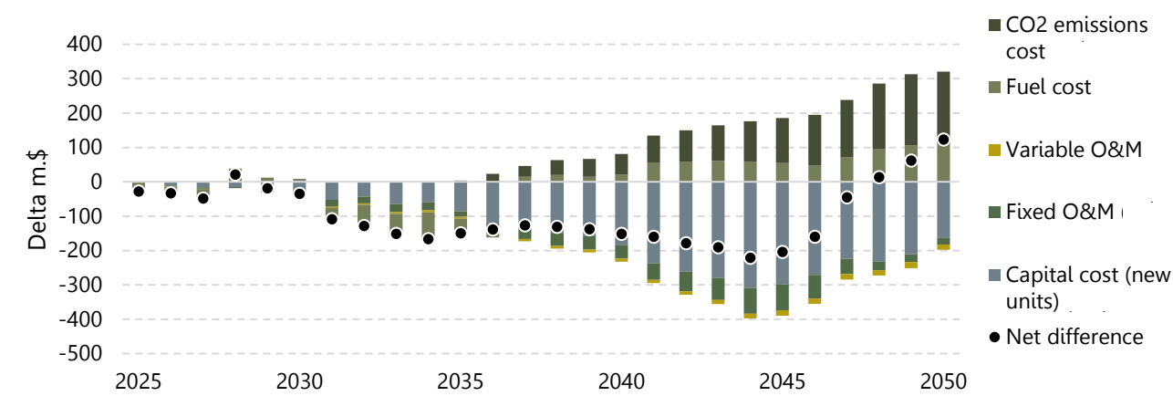
Figure 77: Difference in system costs between NZE and Baseline including CO 2 cost. Positive values mean lower system costs in NZE.
