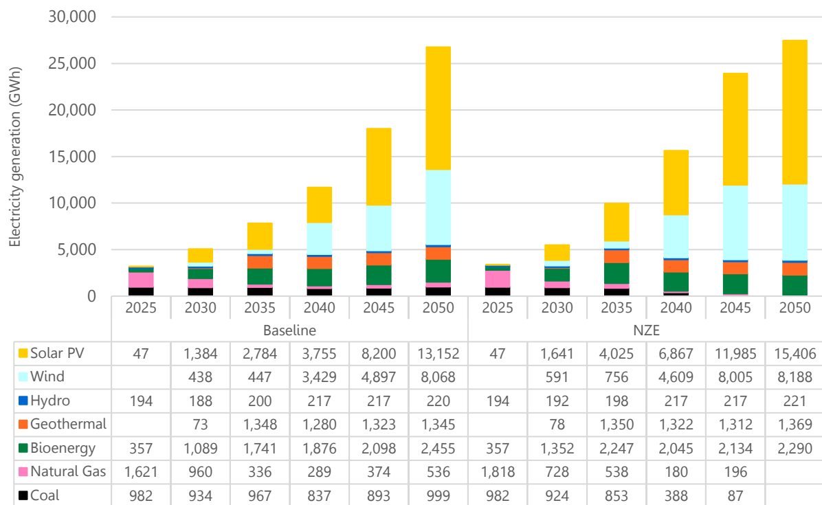
Figure 6: Electricity generation (GWh) for NTB in the two main scenarios.
