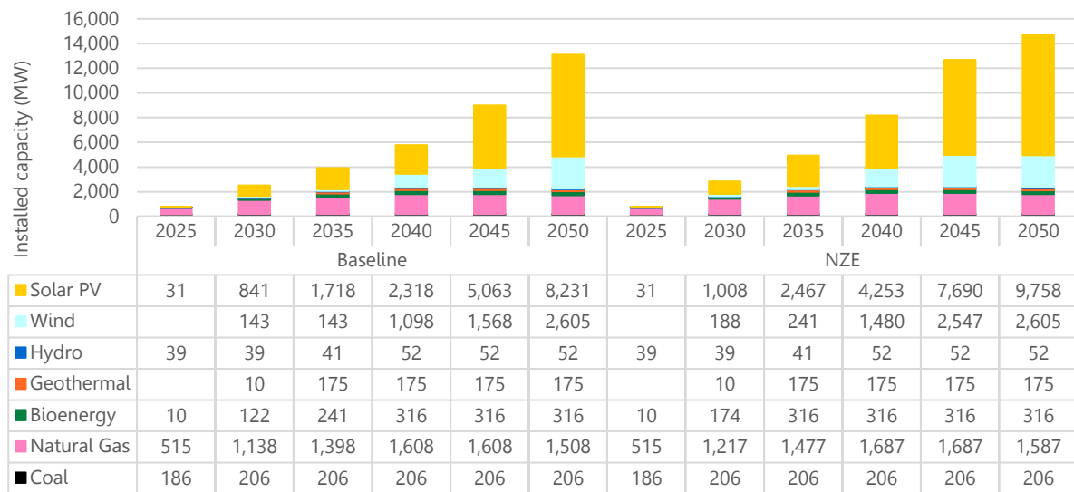
Figure 5: Installed power production capacity (MW) in the two scenarios.
