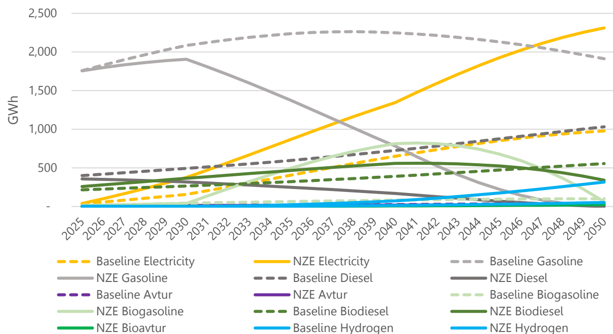
Figure 44. Transportation fuel consumption in Sumbawa
